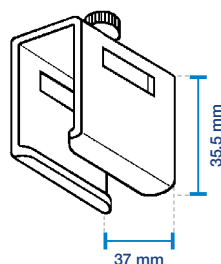
COLLIER COULISSANT
