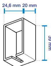
EMBOUT RAIL 700
